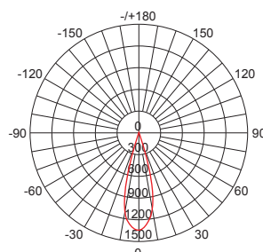
AVERAGE BEAM ANGLE (50%) : 26.3 DEG
